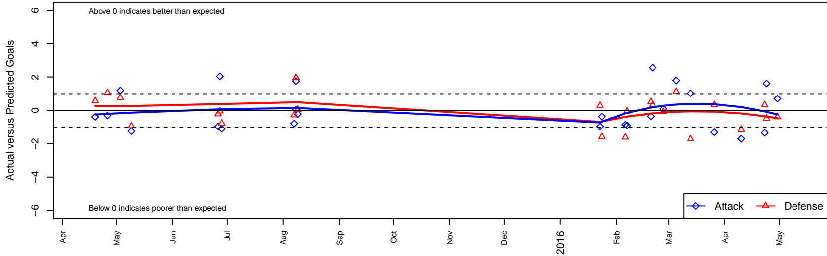
FC Salmon Creek Nemesis Blue G98 Dots are actual minus expected GF (blue circles) and GA (red triangles). Blue line is smoothed change in attack strength. Red is smoothed change in defense strength.
